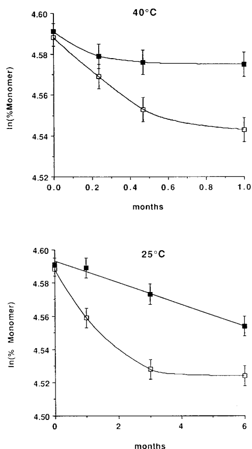
Fig. 3. Representative kinetics for soluble aggregate formation in freeze-dried hGH. Open squares, formulation A; filled squares, formulation D.
