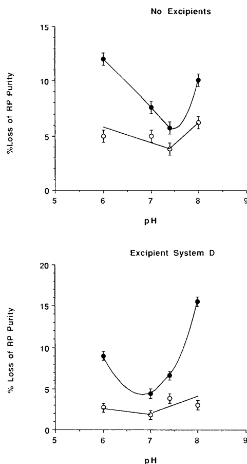
Fig. 9. The effect of pH on loss of reverse-phase purity for freeze-dried hGH. The samples at pH 6, 7, and 8 do not contain buffer. These solutions were adjusted to the appropriate pH by titration with \text{H}_3\text{PO}_4 or NaOH. Filled circles, increase in decomposition after 3 weeks at 40°C; open circles, increase in decomposition after 2 months at 25°C.
