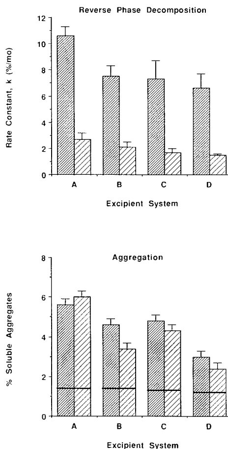
Fig. 6. The effect of excipients on the stability of freeze-dried hGH. The solid horizontal lines in the bottom graph denote the initial level of aggregates in the freeze-dried samples. Reverse-phase decomposition: dark shading, 40°C; light shading, 25°C. Aggregation: dark shading, 3 weeks at 40°C; light shading, 2 months at 25°C.
